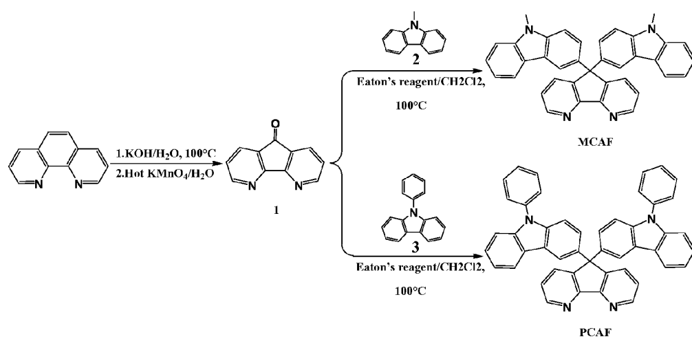
Figure 6. Syntheses of compound 11 (MCAF) and compound 12 (PCAF).
