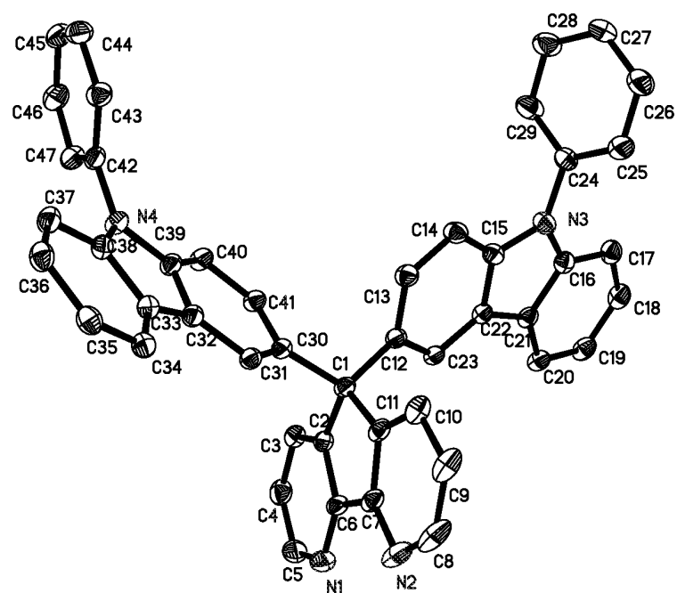
Figure 7. ORTEP diagram of compound 12.
